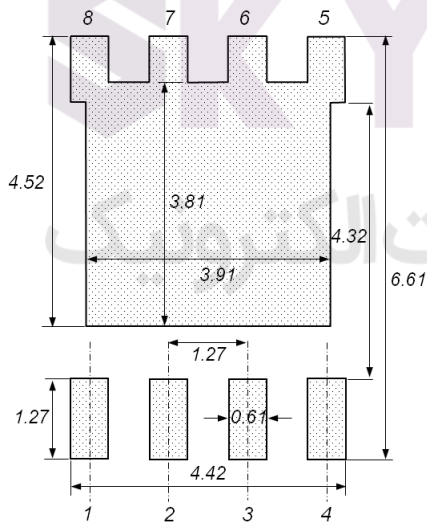
Land Pattern
