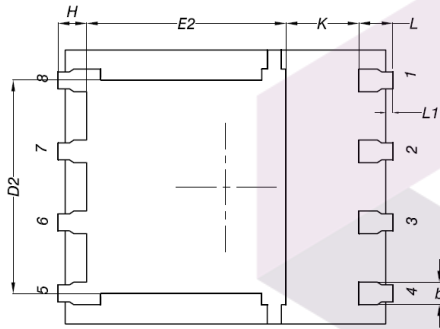
BACKSIDE VIEW
